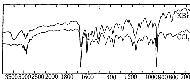
Fig. 1. Infrared spectra of ternstroemiananthin (I).
